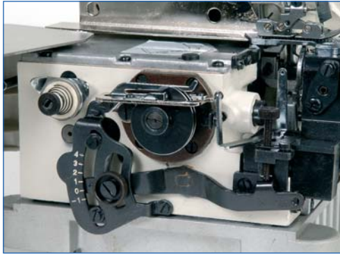
External adjustment differential feed mechanism
